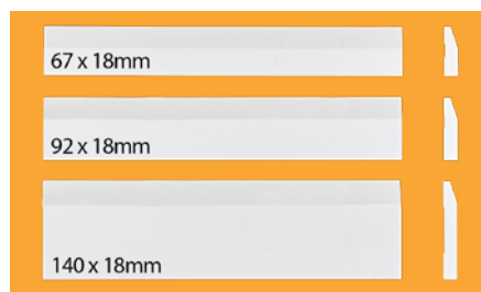
Splayed DSA23
